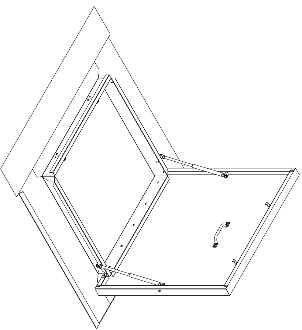
ISOMETRIC VIEW
