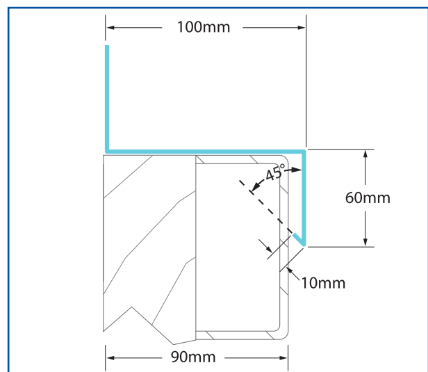
CM (Curb Mount) - Curb Mount (Steel/Timber)
