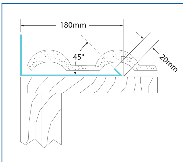
TU (Tile Uprand) - Tile
