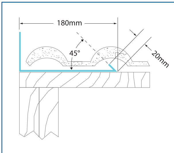
TU (Tile Upstand) - Tile
