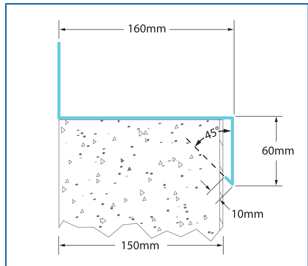
HB (Hob) - Hob Mount (Concrete)
