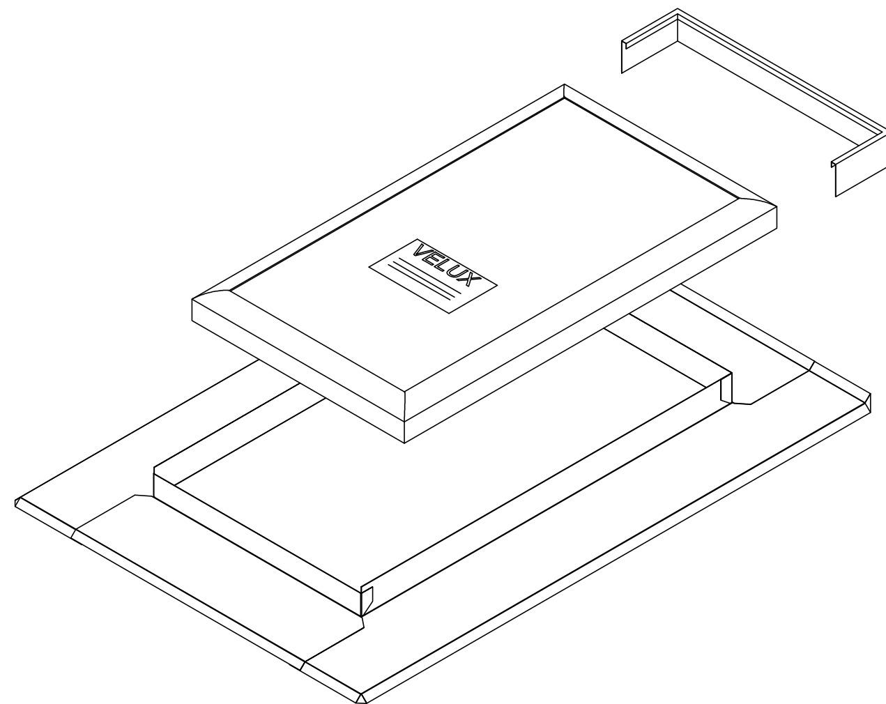
ISOMETRIC VIEW
